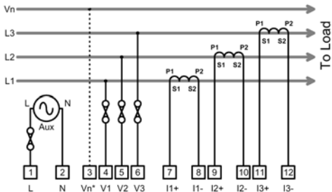
3-Phase 3 or 4-Wire (*Optional Neutral)
